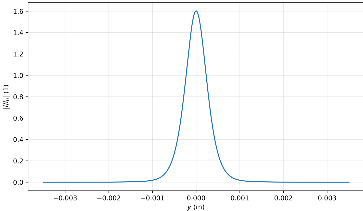
Intensity profile I(x=0, y, z=2.707)/I_0 , P_{in}=0.9P_{cr} , artificial time
